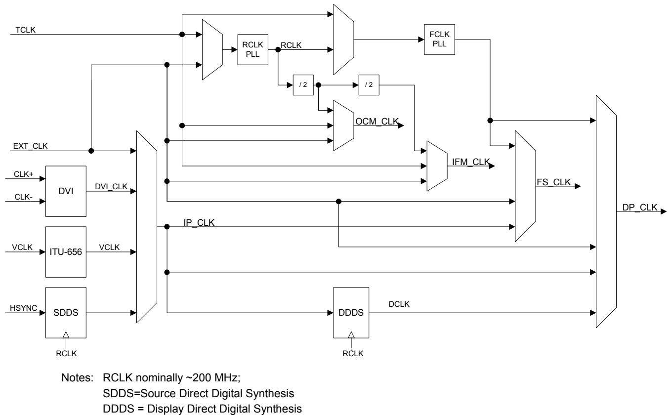
Figure 8. Internal Clock Sources
