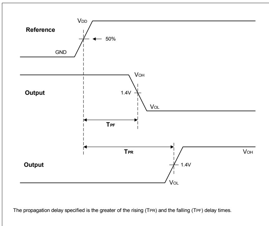
Figure 62. Propagation Delay Reference Levels
