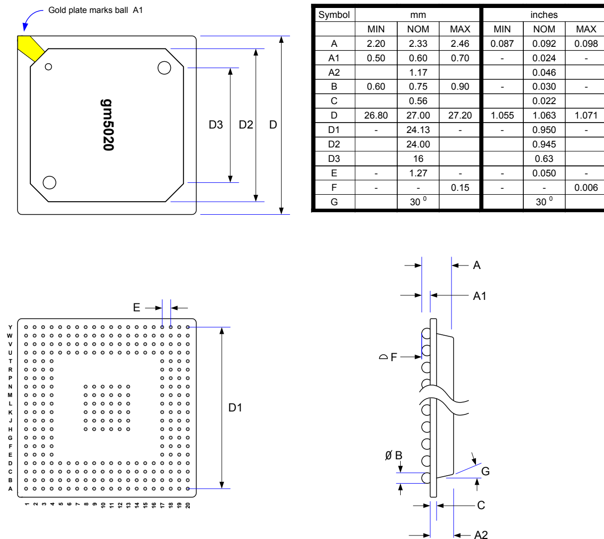
Figure 63. gm5020 292-pin PBGA
