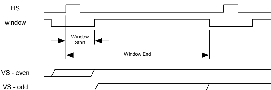
Figure 26. ODD/EVEN Field Detection
