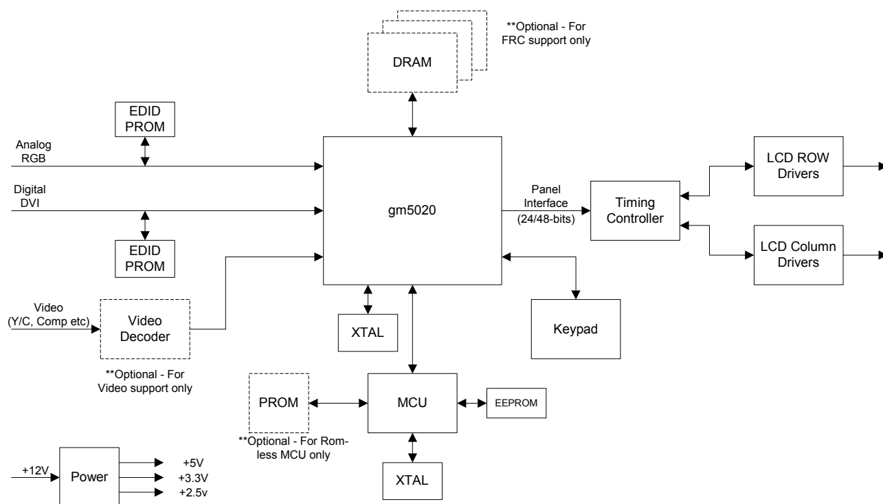
Figure 1. gm5020 System Design Example
