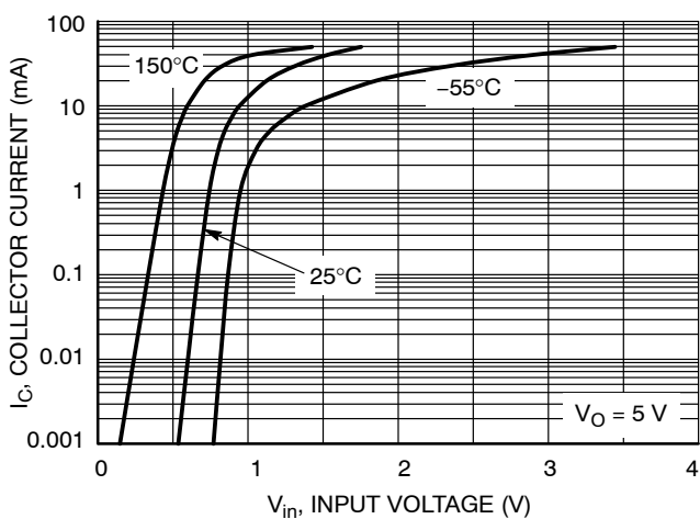
Figure 75. Output Current vs. Input Voltage
