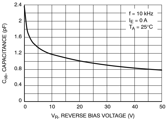
Figure 74. Output Capacitance
