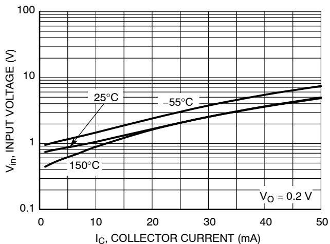
Figure 76. Input Voltage vs. Output Current
