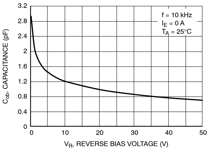
Figure 69. Output Capacitance
