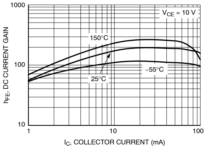
Figure 68. DC Current Gain
