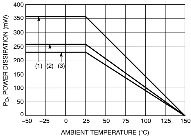
Figure 66. Derating Curve
