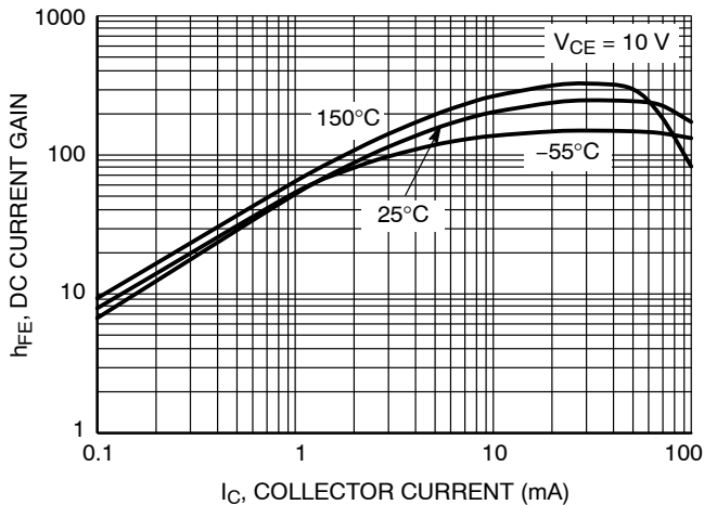
Figure 73. DC Current Gain
