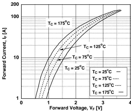
Figure 21. Forward Characteristics
