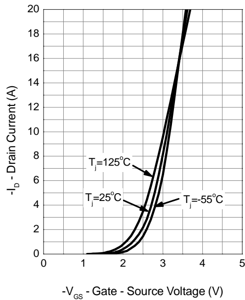
Transfer Characteristics
