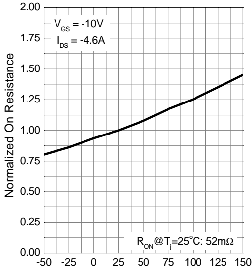
T_J - Junction Temperature ( ^{\circ}C )
