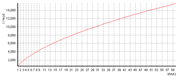
电流-光强曲线 Current-Luminous intensity Curve
