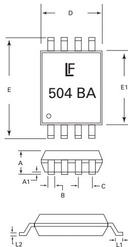
SP0504BAATG - TSSOP-8
