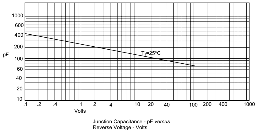
Figure 3 Junction Capacitance
