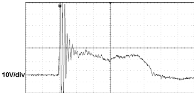
ESD clamping voltage (IEC61000-4-2 +8KV contact)
